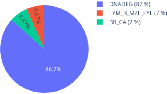
Neighbors in UMAP for 209555540125_R08C01 reference: AllIDATv2_20210804_HPAP_Sarc.xlsx (19967 cases), 0 CpGs
