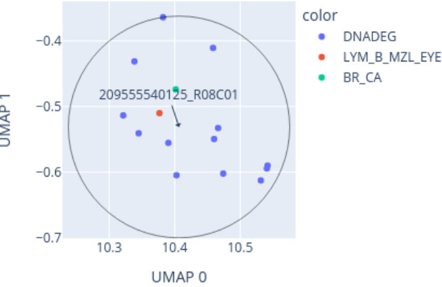
Close-up of UMAP for 209555540125_R08C01 reference: AllIDATv2_20210804_HPAP_Sarc.xlsx (19967 cases), 0 CpGs
