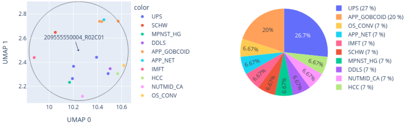
Close-up of UMAP for 209555550004_R02C01 reference: AllIDATv2_20210804_HPAP_Sarc.xlsx (19967 cases), 0 CpGs
