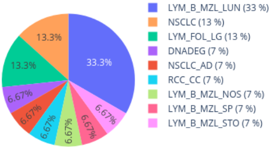
Neighbors in UMAP for 209555550005_R08C01 reference: AllIDATv2_20210804_HPAP_Sarc.xlsx (19967 cases), 0 CpGs
