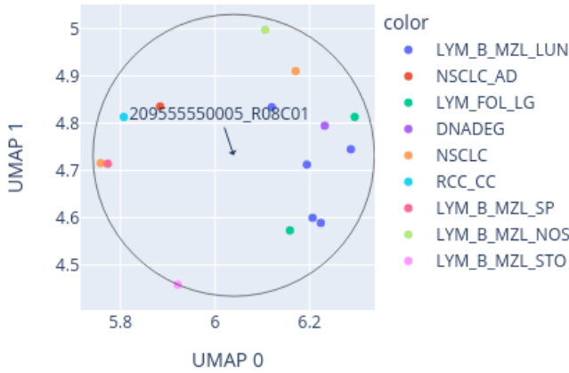
Close-up of UMAP for 209555550005_R08C01 reference: AllIDATv2_20210804_HPAP_Sarc.xlsx (19967 cases), 0 CpGs
