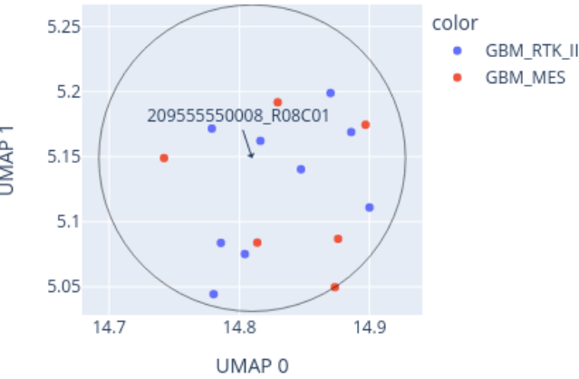
Close-up of UMAP for 209555550008_R08C01 reference: AllIDATv2_20210804_HPAP_Sarc.xlsx (19967 cases), 0 CpGs
