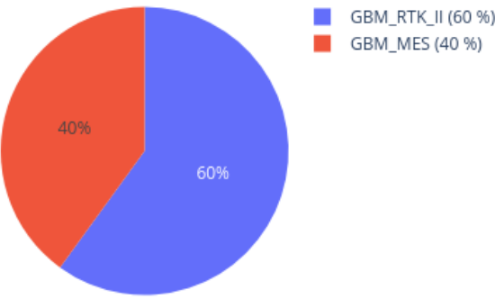
Neighbors in UMAP for 209555550008_R08C01 reference: AllIDATv2_20210804_HPAP_Sarc.xlsx (19967 cases), 0 CpGs
