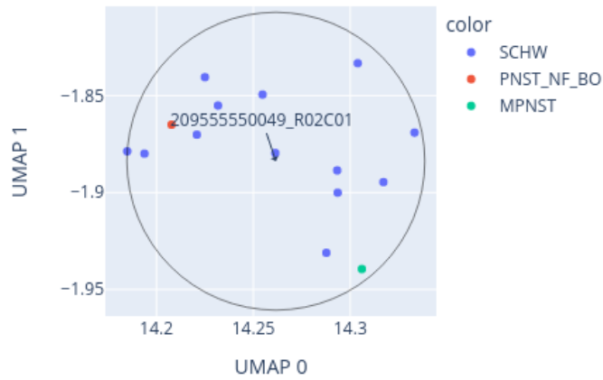
Close-up of UMAP for 209555550049_R02C01 reference: AllIDATv2_20210804_HPAP_Sarc.xlsx (19967 cases), 0 CpGs
