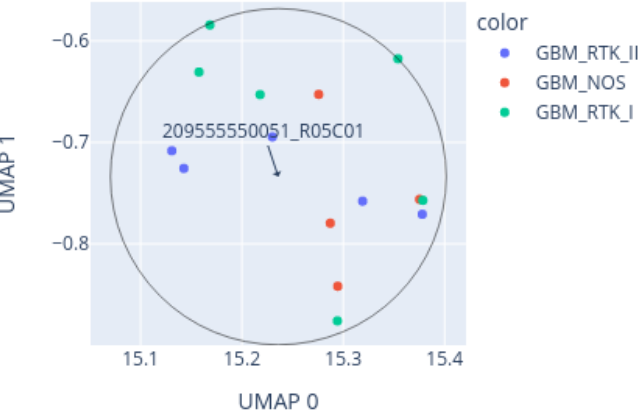
Close-up of UMAP for 209555550051_R05C01 reference: AllIDATv2_20210804_HPAP_Sarc.xlsx (19967 cases), 0 CpGs
