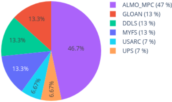
Neighbors in UMAP for 209555550066_R05C01 reference: AllIDATv2_20210804_HPAP_Sarc.xlsx (19967 cases), 0 CpGs
