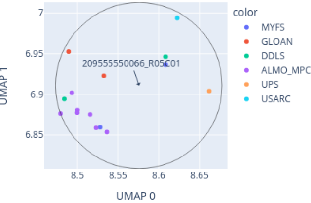
Close-up of UMAP for 209555550066_R05C01 reference: AllIDATv2_20210804_HPAP_Sarc.xlsx (19967 cases), 0 CpGs
