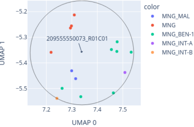
Close-up of UMAP for 209555550073_R01C01 reference: AllIDATv2_20210804_HPAP_Sarc.xlsx (19967 cases), 0 CpGs
