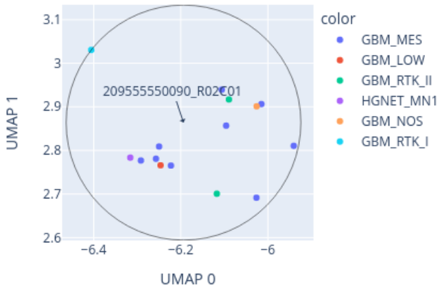
Close-up of UMAP for 209555550090_R02C01 reference: AllIDATv2_20210804_HPAP_Sarc.xlsx (19967 cases), 0 CpGs
