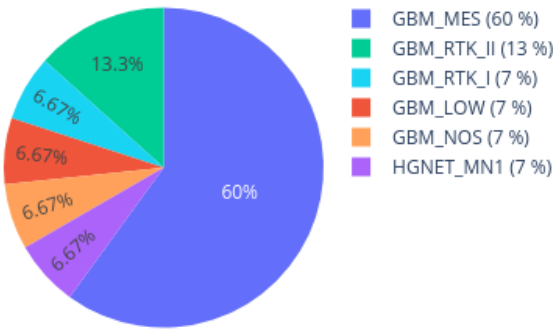
Neighbors in UMAP for 209555550090_R02C01 reference: AllIDATv2_20210804_HPAP_Sarc.xlsx (19967 cases), 0 CpGs
