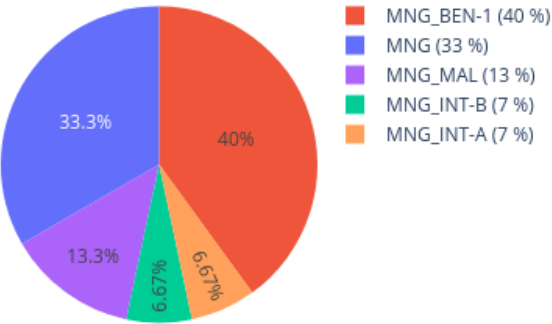
Neighbors in UMAP for 209555550090_R07C01 reference: AllIDATv2_20210804_HPAP_Sarc.xlsx (19967 cases), 0 CpGs
