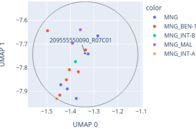
Close-up of UMAP for 209555550090_R07C01 reference: AllIDATv2_20210804_HPAP_Sarc.xlsx (19967 cases), 0 CpGs
