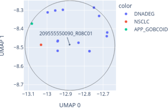
Close-up of UMAP for 209555550090_R08C01 reference: AllIDATv2_20210804_HPAP_Sarc.xlsx (19967 cases), 0 CpGs
