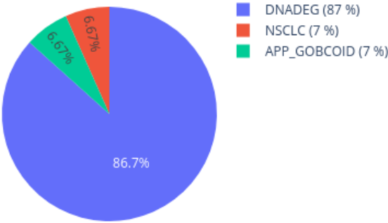
Neighbors in UMAP for 209555550090_R08C01 reference: AllIDATv2_20210804_HPAP_Sarc.xlsx (19967 cases), 0 CpGs
