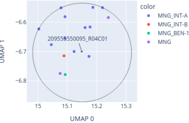
Close-up of UMAP for 209555550095_R04C01 reference: AllIDATv2_20210804_HPAP_Sarc.xlsx (19967 cases), 0 CpGs
