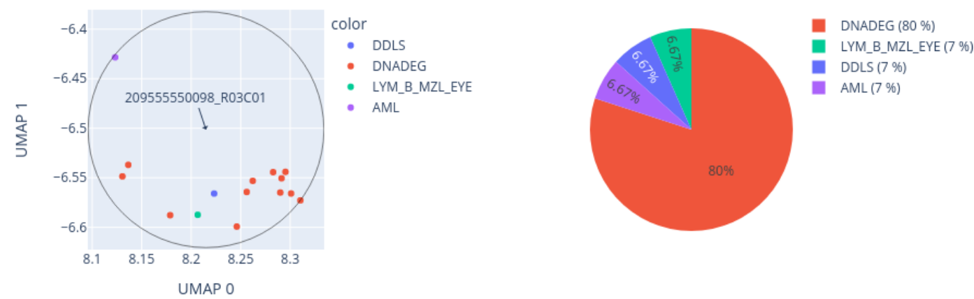
Close-up of UMAP for 209555550098_R03C01 reference: AllIDATv2_20210804_HPAP_Sarc.xlsx (19967 cases), 0 CpGs
