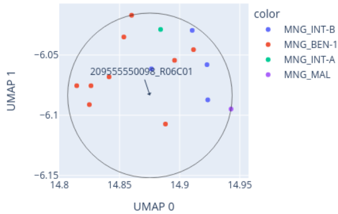
Close-up of UMAP for 209555550098_R06C01 reference: AllIDATv2_20210804_HPAP_Sarc.xlsx (19967 cases), 0 CpGs
