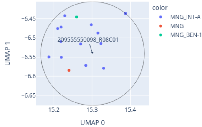
Close-up of UMAP for 209555550098_R08C01 reference: AllIDATv2_20210804_HPAP_Sarc.xlsx (19967 cases), 0 CpGs
