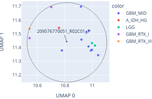
Close-up of UMAP for 209576770051_R02C01_1 reference: AllIDATv2_20210804_HPAP_Sarc.xlsx (19967 cases), 0 CpGs
