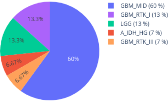
Neighbors in UMAP for 209576770051_R02C01_1 reference: AllIDATv2_20210804_HPAP_Sarc.xlsx (19967 cases), 0 CpGs
