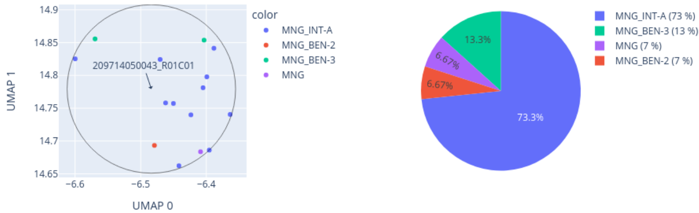
Close-up of UMAP for 209714050043_R01C01 reference: AllIDATv2_20210804_HPAP_Sarc.xlsx (19967 cases), 0 CpGs
