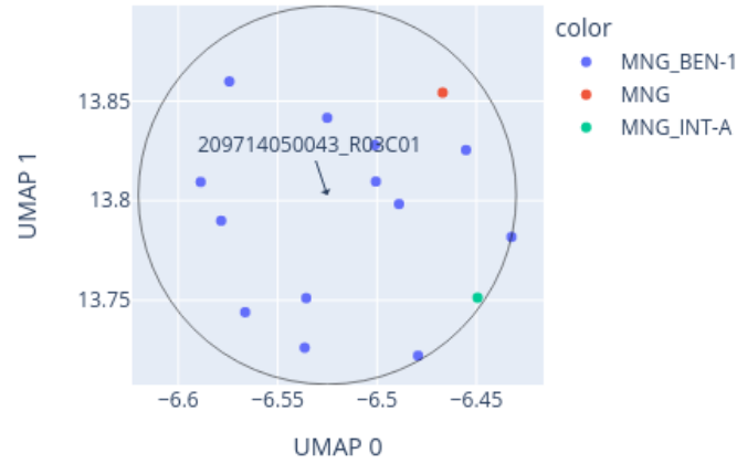
Close-up of UMAP for 209714050043_R03C01 reference: AllIDATv2_20210804_HPAP_Sarc.xlsx (19967 cases), 0 CpGs
