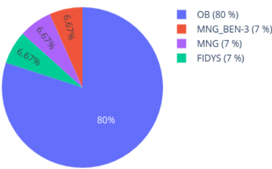
Neighbors in UMAP for 209714050043_R04C01 reference: AllIDATv2_20210804_HPAP_Sarc.xlsx (19967 cases), 0 CpGs
