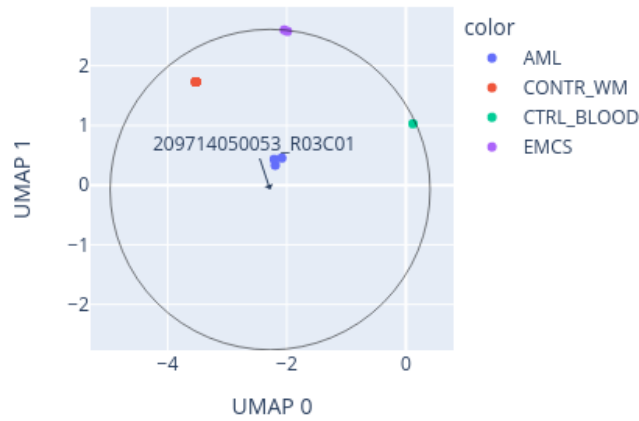
Close-up of UMAP for 209714050053_R03C01 reference: AllIDATv2_20210804_HPAP_Sarc.xlsx (19967 cases), 0 CpGs
