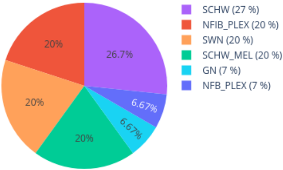
Neighbors in UMAP for 209714050083_R07C01 reference: AllIDATv2_20210804_HPAP_Sarc.xlsx (19967 cases), 0 CpGs
