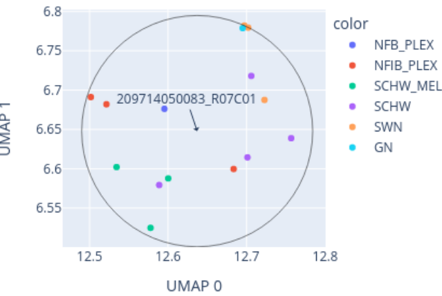
Close-up of UMAP for 209714050083_R07C01 reference: AllIDATv2_20210804_HPAP_Sarc.xlsx (19967 cases), 0 CpGs
