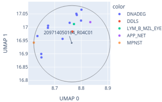
Close-up of UMAP for 209714050164_R04C01 reference: AllIDATv2_20210804_HPAP_Sarc.xlsx (19967 cases), 0 CpGs
