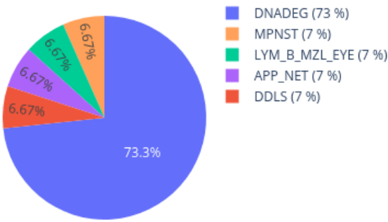
Neighbors in UMAP for 209714050164_R04C01 reference: AllIDATv2_20210804_HPAP_Sarc.xlsx (19967 cases), 0 CpGs
