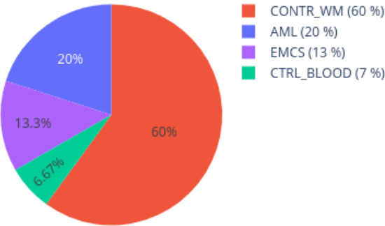
Neighbors in UMAP for 209714050166_R06C01 reference: AllIDATv2_20210804_HPAP_Sarc.xlsx (19967 cases), 0 CpGs
