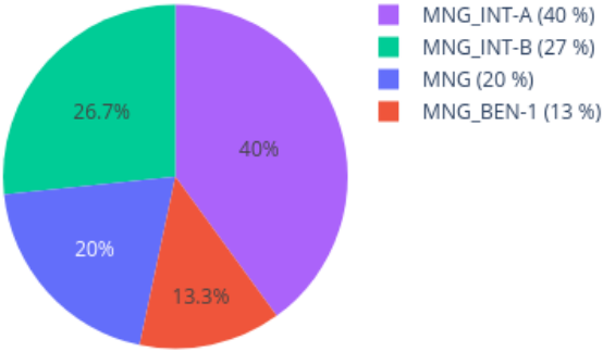
Neighbors in UMAP for 209714050175_R01C01 reference: AllIDATv2_20210804_HPAP_Sarc.xlsx (19967 cases), 0 CpGs
