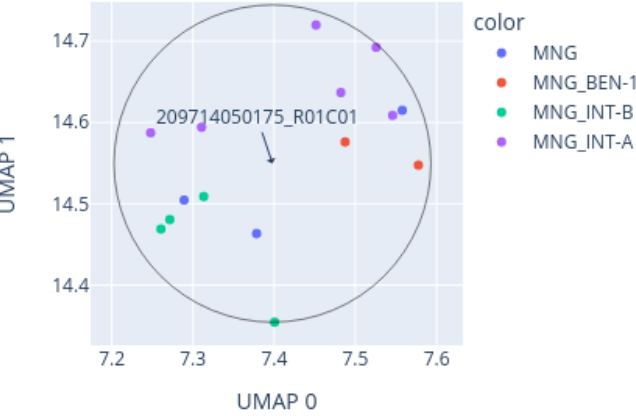
Close-up of UMAP for 209714050175_R01C01 reference: AllIDATv2_20210804_HPAP_Sarc.xlsx (19967 cases), 0 CpGs
