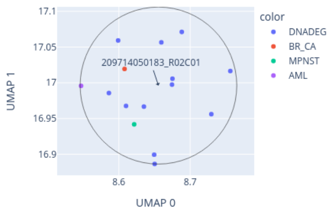
Close-up of UMAP for 209714050183_R02C01 reference: AllIDATv2_20210804_HPAP_Sarc.xlsx (19967 cases), 0 CpGs
