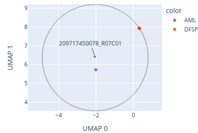
Close-up of UMAP for 209717450078_R07C01 reference: AllIDATv2_20210804_HPAP_Sarc.xlsx (19967 cases), 0 CpGs
