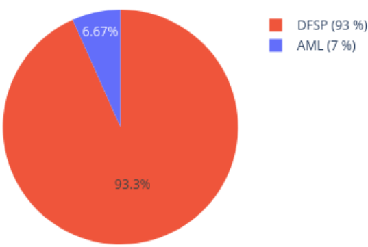
Neighbors in UMAP for 209717450078_R07C01 reference: AllIDATv2_20210804_HPAP_Sarc.xlsx (19967 cases), 0 CpGs
