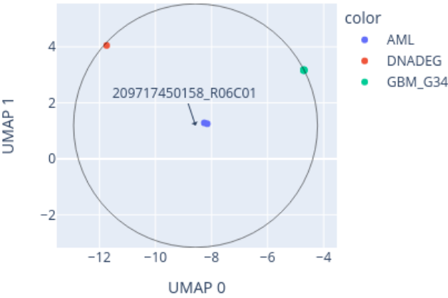
Close-up of UMAP for 209717450158_R06C01 reference: AllIDATv2_20210804_HPAP_Sarc.xlsx (19967 cases), 0 CpGs
