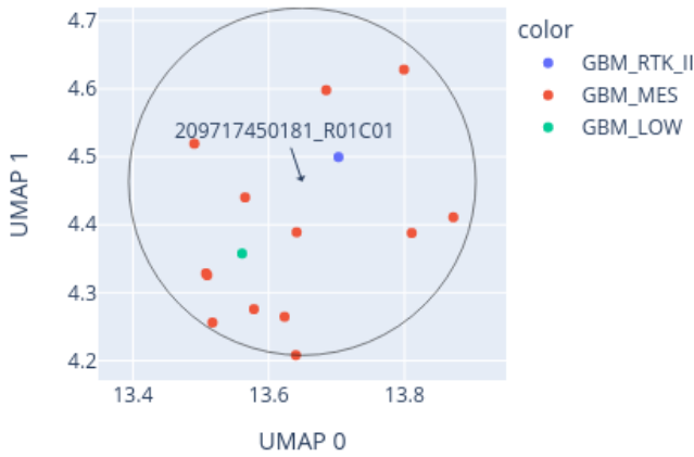
Close-up of UMAP for 209717450181_R01C01 reference: AllIDATv2_20210804_HPAP_Sarc.xlsx (19967 cases), 0 CpGs
