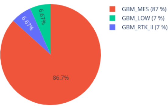
Neighbors in UMAP for 209717450181_R01C01 reference: AllIDATv2_20210804_HPAP_Sarc.xlsx (19967 cases), 0 CpGs
