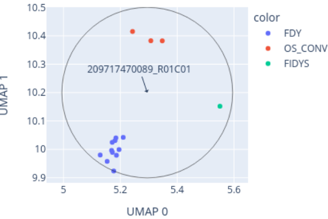
Close-up of UMAP for 209717470089_R01C01 reference: AllIDATv2_20210804_HPAP_Sarc.xlsx (19967 cases), 0 CpGs
