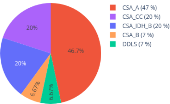
Neighbors in UMAP for 209717470089_R03C01 reference: AllIDATv2_20210804_HPAP_Sarc.xlsx (19967 cases), 0 CpGs
