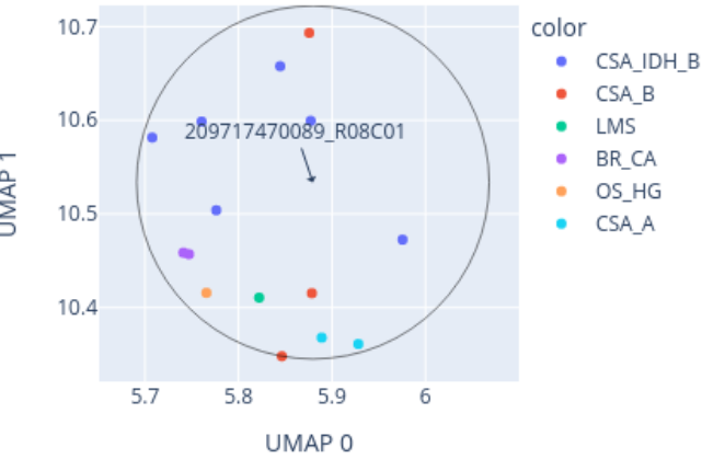
Close-up of UMAP for 209717470089_R08C01 reference: AllIDATv2_20210804_HPAP_Sarc.xlsx (19967 cases), 0 CpGs
