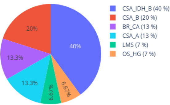
Neighbors in UMAP for 209717470089_R08C01 reference: AllIDATv2_20210804_HPAP_Sarc.xlsx (19967 cases), 0 CpGs
