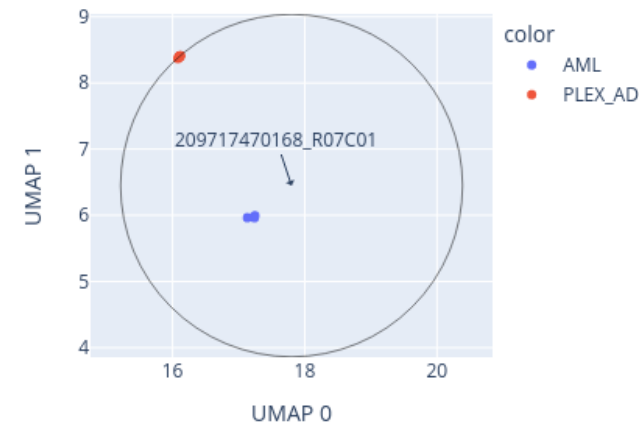
Close-up of UMAP for 209717470168_R07C01 reference: AllIDATv2_20210804_HPAP_Sarc.xlsx (19967 cases), 0 CpGs
