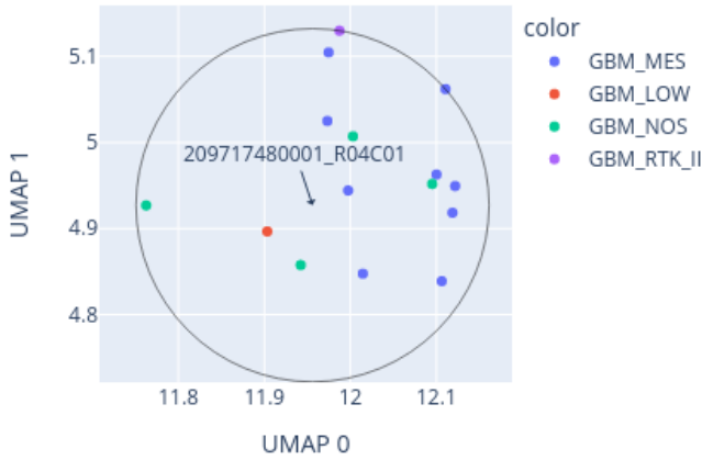
Close-up of UMAP for 209717480001_R04C01 reference: AllIDATv2_20210804_HPAP_Sarc.xlsx (19967 cases), 0 CpGs
