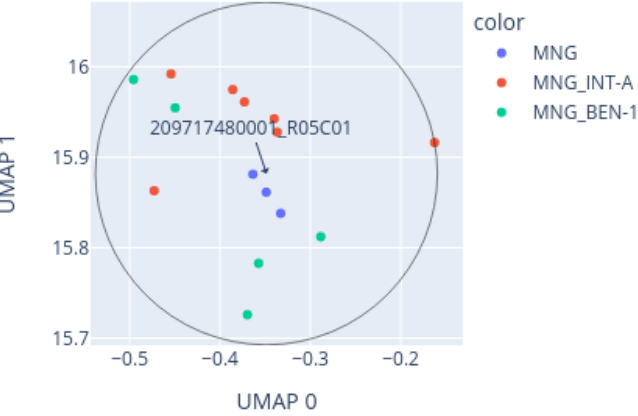
Close-up of UMAP for 209717480001_R05C01 reference: AllIDATv2_20210804_HPAP_Sarc.xlsx (19967 cases), 0 CpGs
