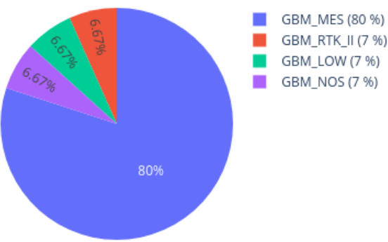
Neighbors in UMAP for 209717480001_R07C01 reference: AllIDATv2_20210804_HPAP_Sarc.xlsx (19967 cases), 0 CpGs
