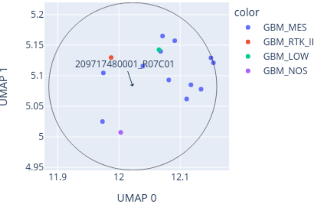
Close-up of UMAP for 209717480001_R07C01 reference: AllIDATv2_20210804_HPAP_Sarc.xlsx (19967 cases), 0 CpGs
