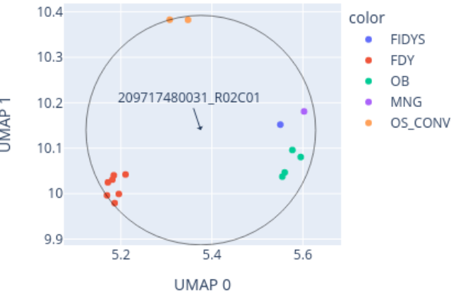
Close-up of UMAP for 209717480031_R02C01 reference: AllIDATv2_20210804_HPAP_Sarc.xlsx (19967 cases), 0 CpGs
