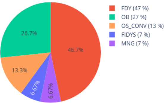
Neighbors in UMAP for 209717480031_R02C01 reference: AllIDATv2_20210804_HPAP_Sarc.xlsx (19967 cases), 0 CpGs
