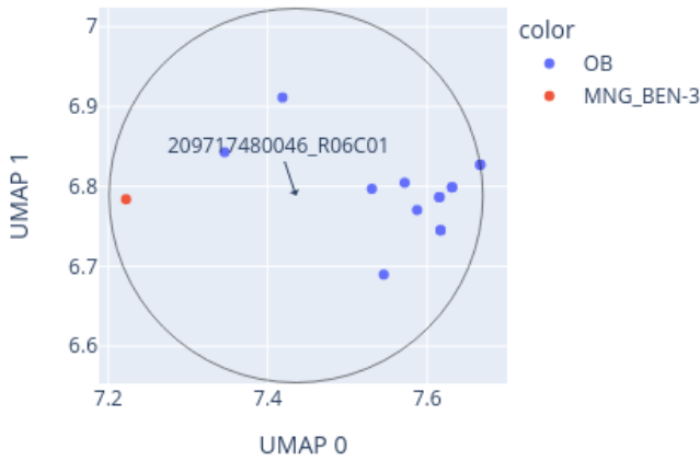
Close-up of UMAP for 209717480046_R06C01 reference: AllIDATv2_20210804_HPAP_Sarc.xlsx (19967 cases), 0 CpGs
