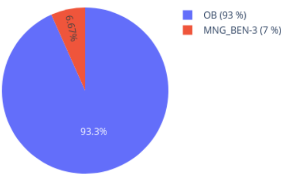
Neighbors in UMAP for 209717480046_R06C01 reference: AllIDATv2_20210804_HPAP_Sarc.xlsx (19967 cases), 0 CpGs
