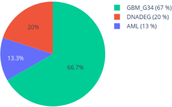
Neighbors in UMAP for 209717480058_R07C01 reference: AllIDATv2_20210804_HPAP_Sarc.xlsx (19967 cases), 0 CpGs
