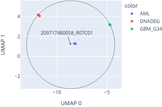
Close-up of UMAP for 209717480058_R07C01 reference: AllIDATv2_20210804_HPAP_Sarc.xlsx (19967 cases), 0 CpGs
