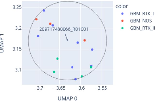
Close-up of UMAP for 209717480066_R01C01 reference: AllIDATv2_20210804_HPAP_Sarc.xlsx (19967 cases), 0 CpGs
