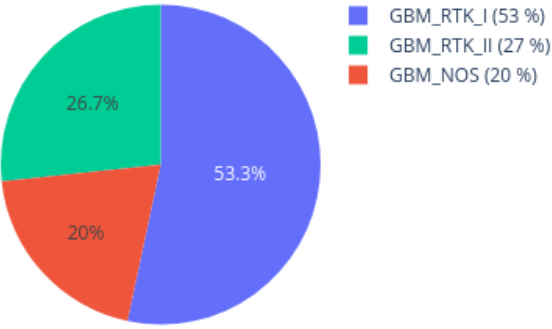
Neighbors in UMAP for 209717480066_R01C01 reference: AllIDATv2_20210804_HPAP_Sarc.xlsx (19967 cases), 0 CpGs
