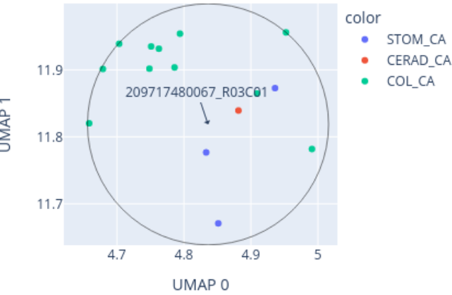
Close-up of UMAP for 209717480067_R03C01 reference: AllIDATv2_20210804_HPAP_Sarc.xlsx (19967 cases), 0 CpGs
