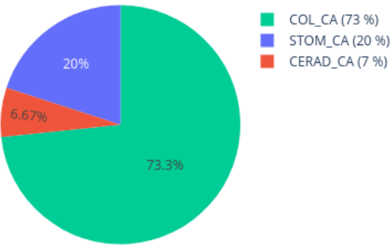
Neighbors in UMAP for 209717480067_R03C01 reference: AllIDATv2_20210804_HPAP_Sarc.xlsx (19967 cases), 0 CpGs
