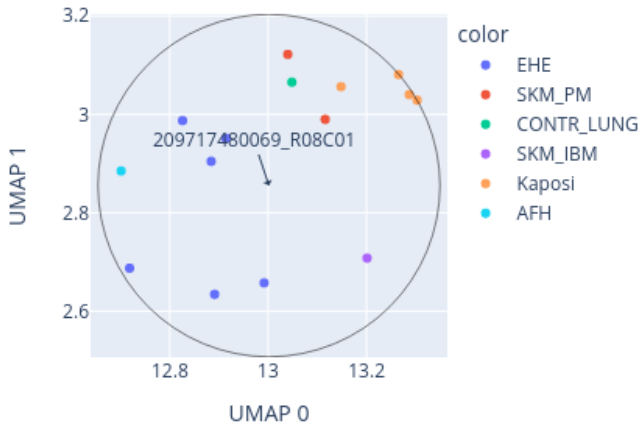
Close-up of UMAP for 209717480069_R08C01 reference: AllIDATv2_20210804_HPAP_Sarc.xlsx (19967 cases), 0 CpGs
