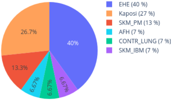
Neighbors in UMAP for 209717480069_R08C01 reference: AllIDATv2_20210804_HPAP_Sarc.xlsx (19967 cases), 0 CpGs
