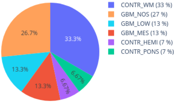
Neighbors in UMAP for 209717480087_R01C01 reference: AllIDATv2_20210804_HPAP_Sarc.xlsx (19967 cases), 0 CpGs
