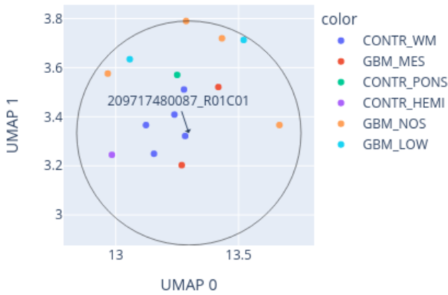
Close-up of UMAP for 209717480087_R01C01 reference: AllIDATv2_20210804_HPAP_Sarc.xlsx (19967 cases), 0 CpGs
