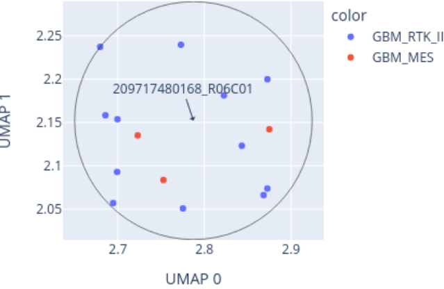
Close-up of UMAP for 209717480168_R06C01 reference: AllIDATv2_20210804_HPAP_Sarc.xlsx (19967 cases), 0 CpGs
