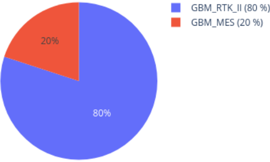
Neighbors in UMAP for 209717480168_R06C01 reference: AllIDATv2_20210804_HPAP_Sarc.xlsx (19967 cases), 0 CpGs
