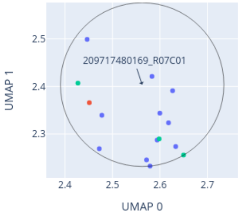
Close-up of UMAP for 209717480169_R07C01 reference: AllIDATv2_20210804_HPAP_Sarc.xlsx (19967 cases), 0 CpGs
