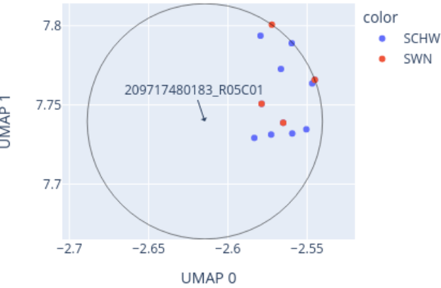
Close-up of UMAP for 209717480183_R05C01 reference: AllIDATv2_20210804_HPAP_Sarc.xlsx (19967 cases), 0 CpGs
