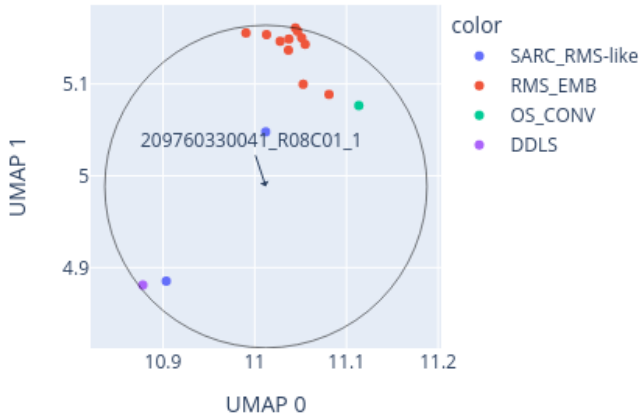
Close-up of UMAP for 209760330041_R08C01_1 reference: AllIDATv2_20210804_HPAP_Sarc.xlsx (19967 cases), 0 CpGs
