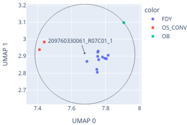
Close-up of UMAP for 209760330061_R07C01_1 reference: AllIDATv2_20210804_HPAP_Sarc.xlsx (19967 cases), 0 CpGs
