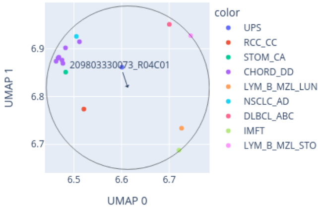
Close-up of UMAP for 209803330073_R04C01 reference: AllIDATv2_20210804_HPAP_Sarc.xlsx (19967 cases), 0 CpGs
