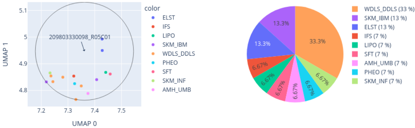
Close-up of UMAP for 209803330098_R05C01 reference: AllIDATv2_20210804_HPAP_Sarc.xlsx (19967 cases), 0 CpGs
