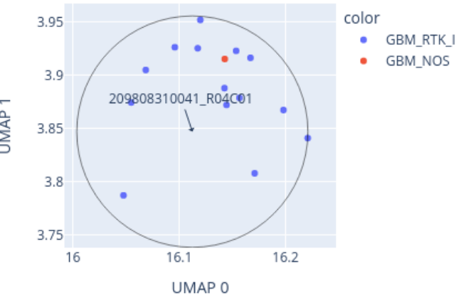
Close-up of UMAP for 209808310041_R04C01 reference: AllIDATv2_20210804_HPAP_Sarc.xlsx (19967 cases), 0 CpGs
